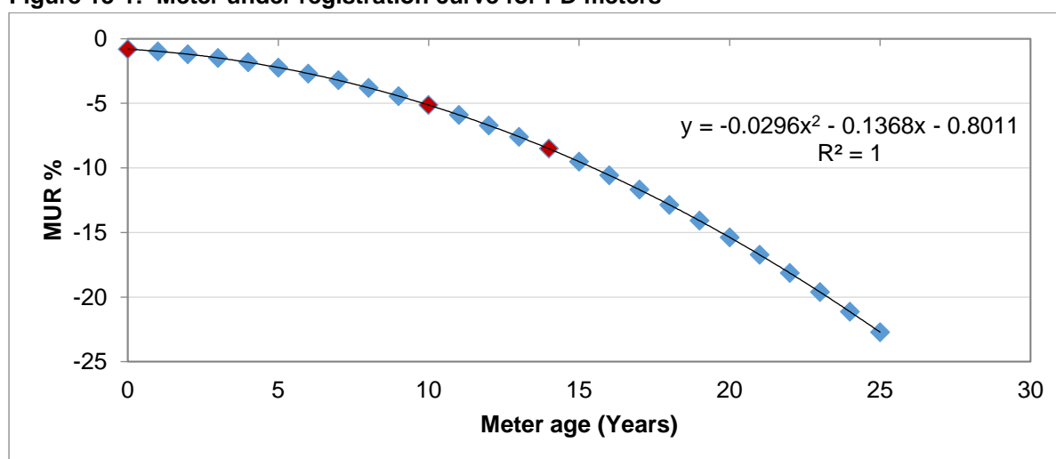
Figure 13-1: Meter under registration curve for PD meters
