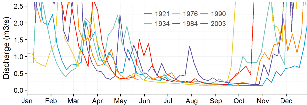
Figure 4-5 Total simulated inflow into impounding reservoirs for the driest years in the historic record (1911-2016)
