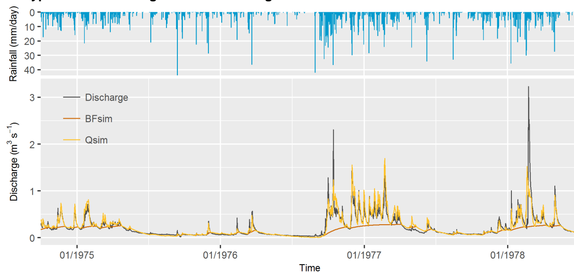
Figure 4-9 Comparison of observed (Discharge) and modelled (Qsim) river discharge for the Currypool stream during the 1975/76 drought event
