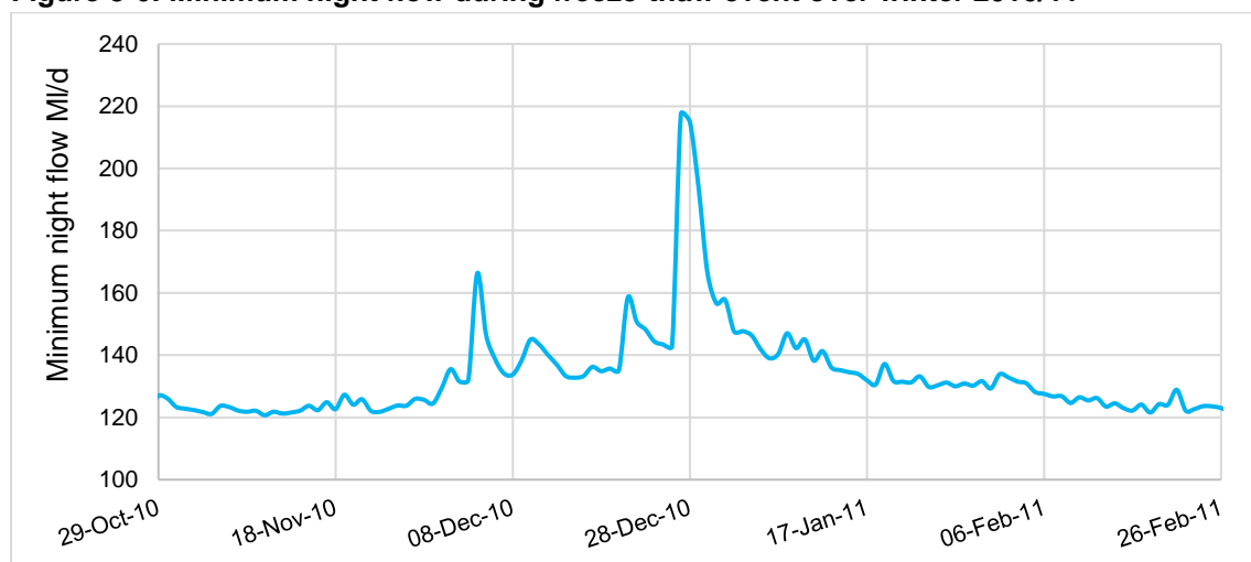
Figure 8-6: Minimum night flow during freeze-thaw event over winter 2010/11
