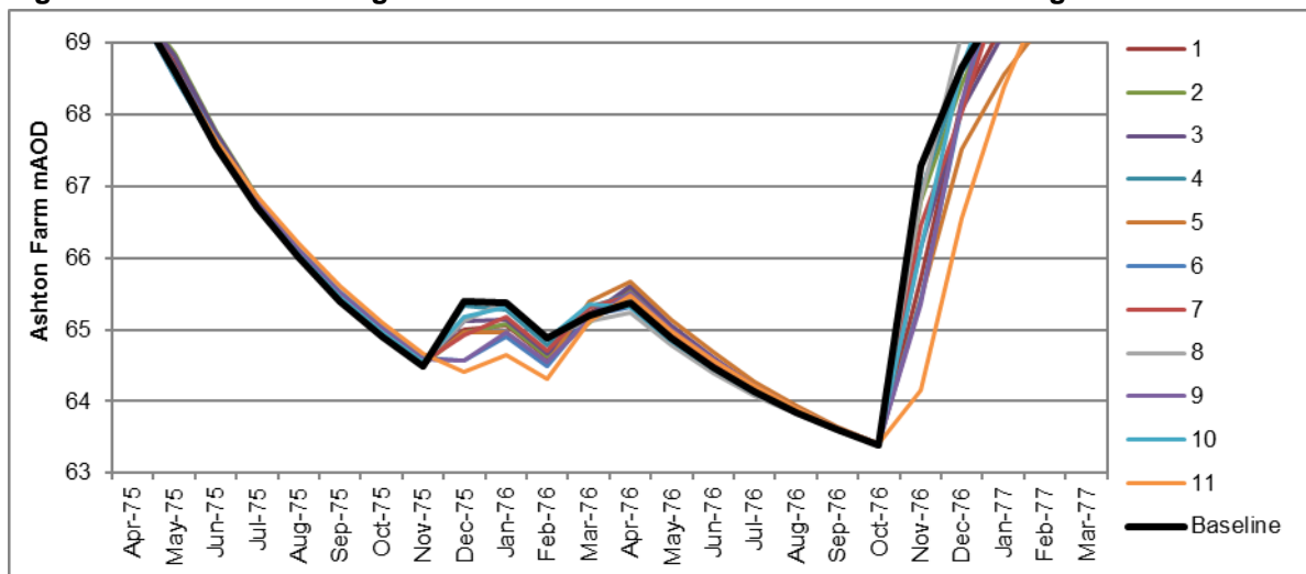
Figure 4-22: Ashton Farm groundwater levels modelled for 11 climate change scenarios
