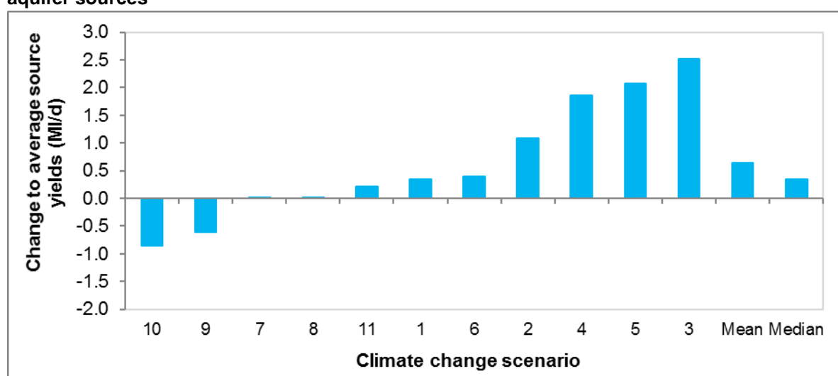
Figure 4-25: Impact of climate change scenarios on the average yield of the Chippenham aquifer sources
