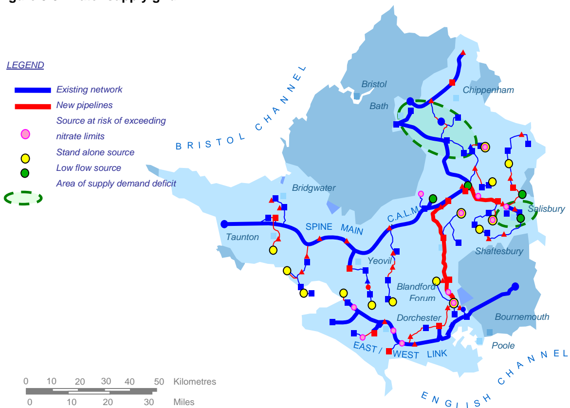
Figure 8-3: Water supply grid
