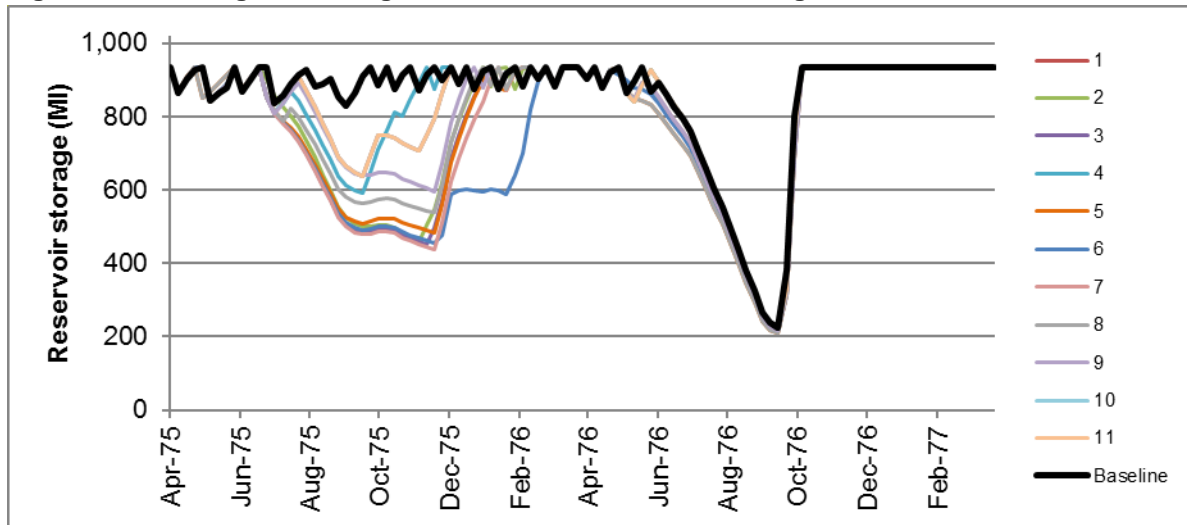
Figure 4-26: Storage in Durleigh Reservoir under climate change scenarios
