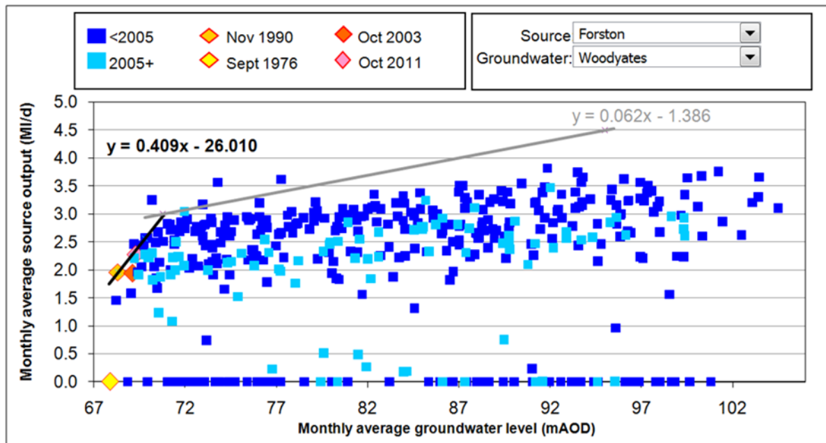
Figure 4-7 Example correlation between monthly source output and Woodyates groundwater level for Forston
