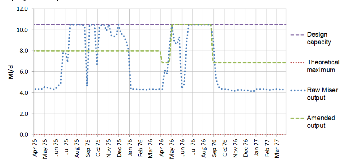
Figure 4-15: Black Lane source outputs from Miser and the amended values used for defining deployable output
