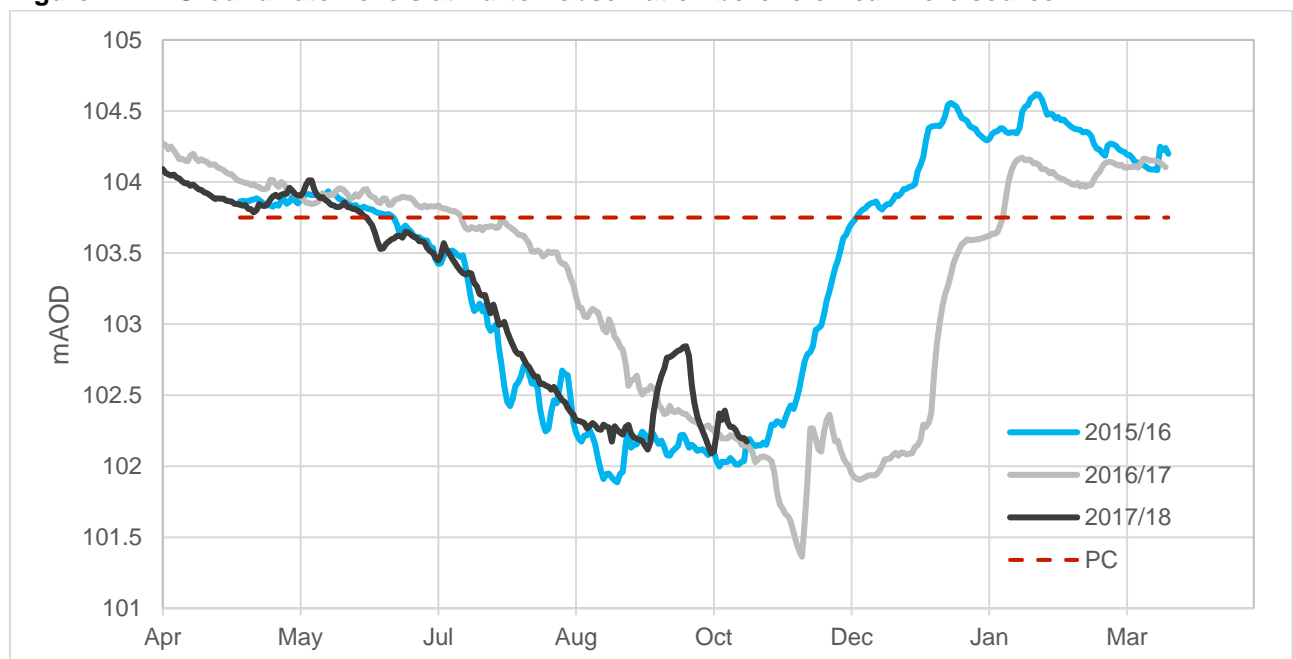
Figure 4-11: Groundwater levels at Burton observation borehole near Mere source
